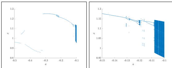
Fig. 5. Gotthans-Petržela model: Bifurcation diagram of x with respect to a : left a \in (-0.5, -0.1) , right a \in (-0.15, -0.1) .
