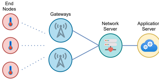
Fig. 1. Standard LoRaWAN architecture.
