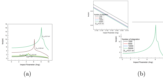
Fig. 5: The collision time \tau as a function of the collision energy E_{\text{coll}} , the impact parameter b and different numbers of integration steps at as obtained for the ground state of the Ar_2^+ dimer.
