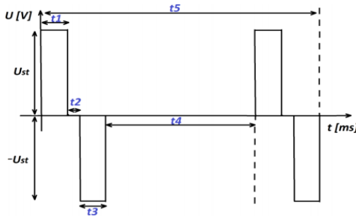
Fig. 1. Design of the biphasic stimulation pulse
