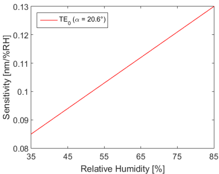
Fig. 11. Sensitivity of TE_0 mode measured at the external angle of incidence \alpha = 20.6^\circ .
