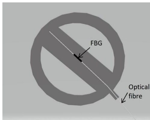
Fig.3. 3D model of the sensor.
