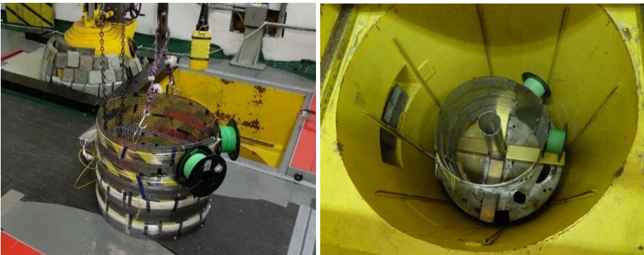
Fig. 1. Optical fiber samples were prepared on stainless steel performed drum, which was placed inside irradiation chamber.
